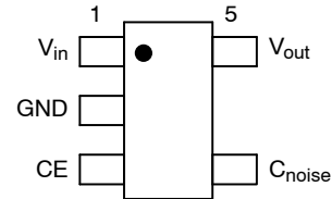
TSOP-5 (Top View)
